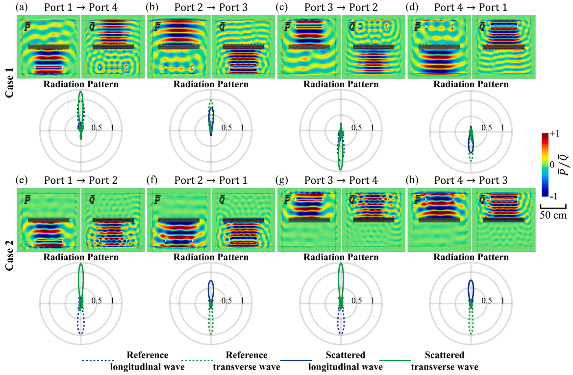
Fig. 4. Collective response of the designed bidirectional mode conversion meta-atom and corresponding radiation pattern. The transmission meta-atom of Case 1 under the excitation of (a) longitudinal wave incidence from the lower side, (b) transverse wave incidence from the lower side, (c) longitudinal wave incidence from the upper side, and (d) transverse wave incidence from the upper side. The reflection meta-atom of Case 2 under the excitation of (e) longitudinal wave incidence from the lower side, (f) transverse wave incidence from the lower side, (g) longitudinal wave incidence from the upper side, and (h) transverse wave incidence from the upper side.
