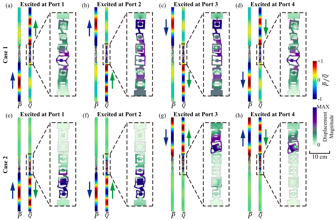
Fig. 3. Structure design of the meta-atom and responses for transmission and reflection bidirectional mode conversion. (a) The response of transmission meta-atom under longitudinal waves incident from the lower side, i.e. excited at port 1. (b) The response of transmission meta-atom under transverse waves incident from the lower side, i.e. excited at port 2. (c) The response of transmission meta-atom under longitudinal waves incident from the upper side, i.e. excited at port 3. (d) The response of transmission meta-atom under transverse waves incident from the upper side, i.e. excited at port 4. (e) The response of reflection meta-atom under longitudinal waves incident from the lower side, i.e. excited at port 1. (f) The response of reflection meta-atom under transverse waves incident from the lower side, i.e. excited at port 2. (g) The response of reflection meta-atom under longitudinal waves incident from the upper side, i.e. excited at port 3. (h) The response of reflection meta-atom under transverse waves incident from the upper side, i.e. excited at port 4.
