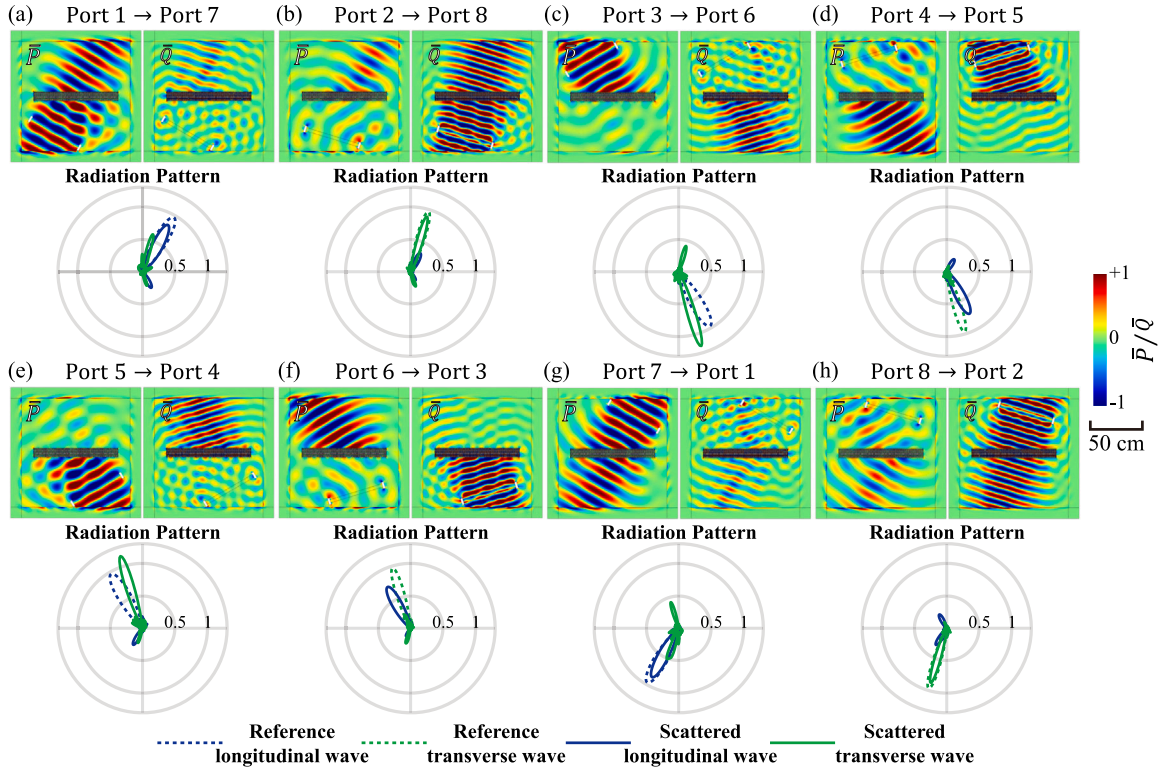
Fig. 6. Collective response of the designed extremely asymmetric meta-atom and corresponding radiation pattern. (a) Response without mode conversion under an incident longitudinal wave from the lower left side. (b) Response without mode conversion under the incident transverse wave from the lower left side. (c) Response with mode conversion under the incident longitudinal wave from the upper left side. (d) Response with mode conversion under the incident transverse wave from the upper left side. (e) Response with mode conversion under the incident longitudinal wave from the lower right side. (f) Response with mode conversion under the incident transverse wave from the upper right side. (g) Response without mode conversion under the incident longitudinal wave from the upper right side. (h) Response without mode conversion under the incident transverse wave from the upper right side.
