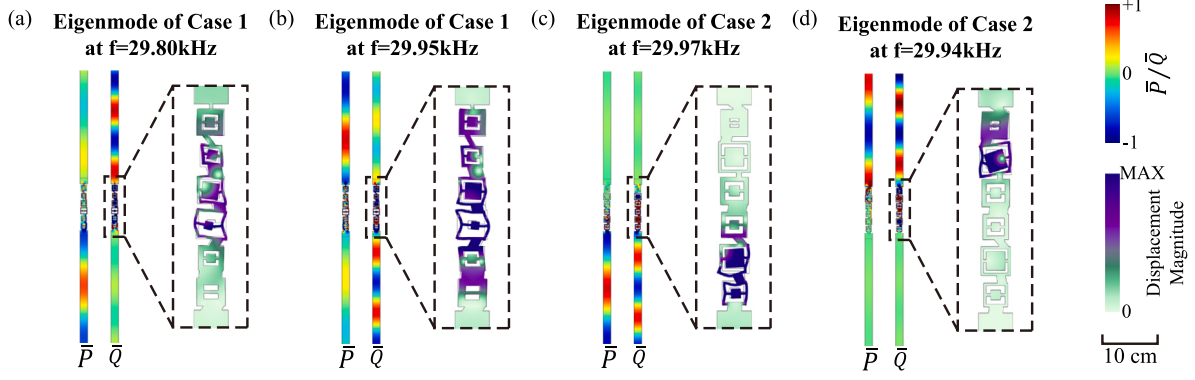
Fig. 8. Eigenmodes of the designed meta-atom. (a) The eigenmode of the meta-atom in Case 1 at 29.80 kHz. (b) The eigenmode of the meta-atom in Case 1 at 29.95 kHz. (c) The eigenmode of the meta-atom in Case 2 at 29.97 kHz. (d) The eigenmode of the meta-atom in Case 2 at 29.94 kHz.
