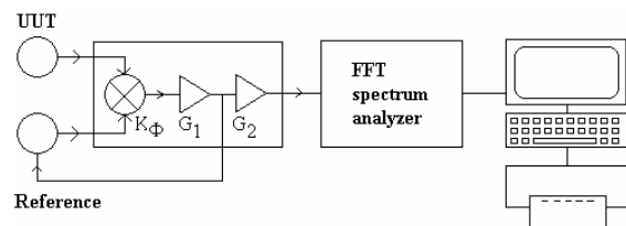
Fig. 3. Principle of the phase noise calibration.
