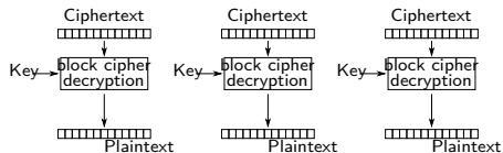
Electronic Codebook (ECB) mode decryption
