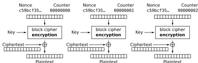
Counter (CTR) mode decryption
